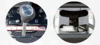
Optional transmission
